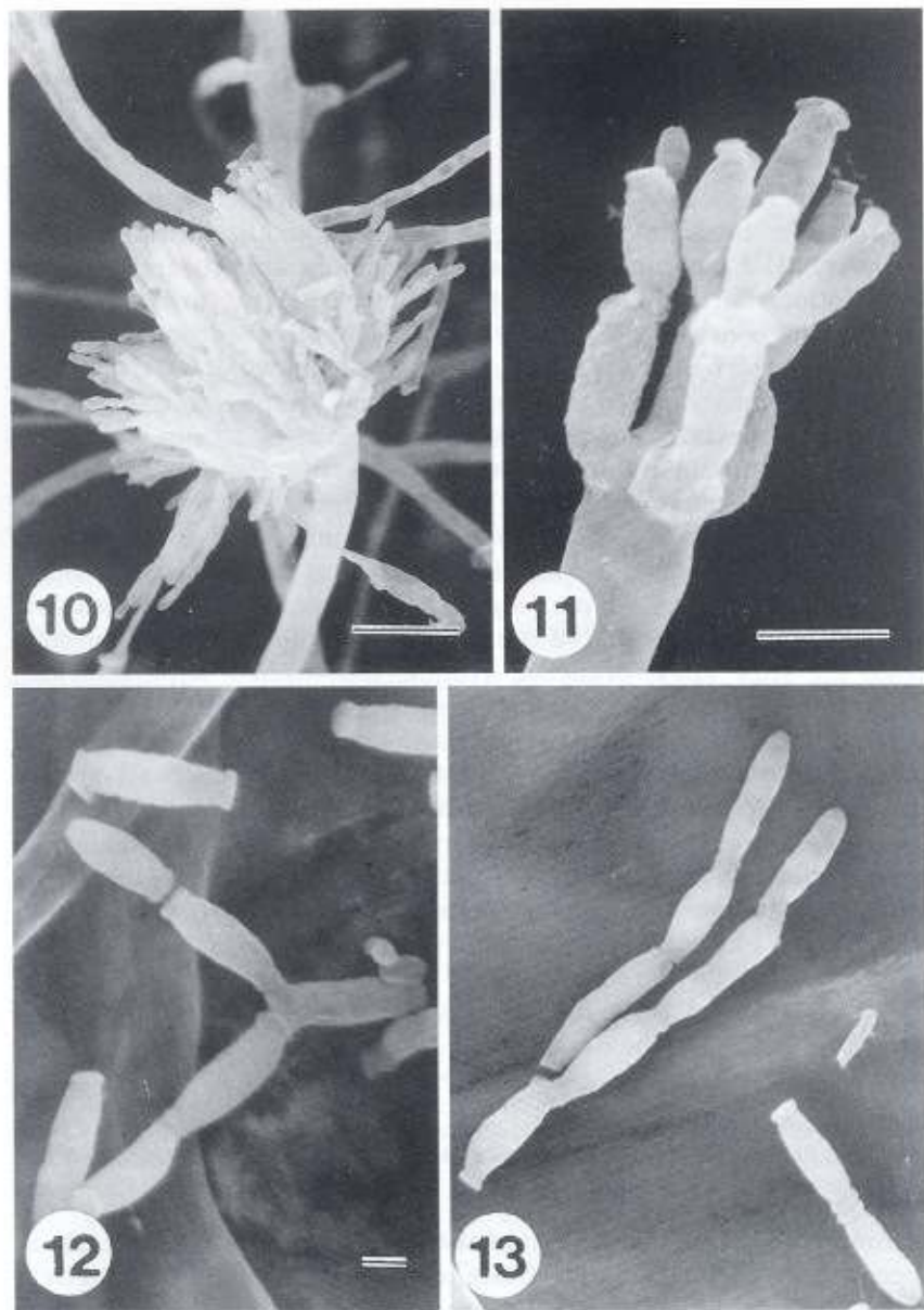
Figs. 10-13. - Scanning electron micrographs of Lauriomyces bellulus . - 10. conidiophore with conidia arranged in dry heads (bar = 10 \mu\text{m} ). - 11. conidiogenous apparatus showing conidiophore branches (bar = 5 \mu\text{m} ). - 12 & 13. branched conidial chains showing thickened conidial dehiscence scars (bar = 1 \mu\text{m} ).
