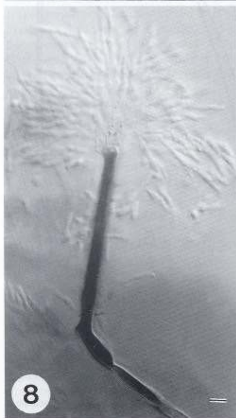
Figs. 7-9. - Light micrographs of Lauriomyces bellulus . - 7. mononematous conidiophores (bar = 15 \mu m). - 8, 9. conidiophore arising directly from the mycelium and giving rise to hyaline, non-septate, branched conidial chains (bar = 5 \mu m).
