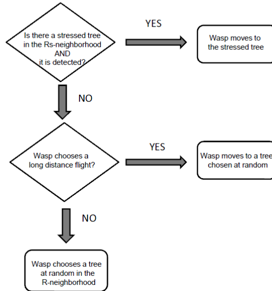
FIGURE 2. Flow-chart for the decision-making process used to simulate wasp dispersal.
