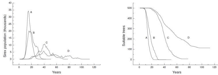
FIGURE 3. Left plate. Outbreaks obtained when long distance dispersal is precluded ( P_{LDD}=0 ). Curves A and B correspond to \tau = 12 , and R=4 and R=2 , respectively (where \tau is the number of trees visited by each wasp during its lifetime, and R is the radius for local dispersal). Curves C and D correspond to \tau=6 , and R=4 and R=2 , respectively. Right plate. Number of susceptible trees during the four simulations (A, B, C, and D). In all cases the initial proportion of susceptible trees ( \rho ) was set to 0.05.
