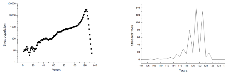
FIGURE 6. Wasp population growth with simulation conditions as in Fig. 3 D ( P_{LDD} = 0.1 , \rho = 0.05 , \tau = 6 , R = 4 ). Later, a phase of slow exponential growth until year 107 is noted, when the first stressed tree appears in the plantation triggering the outbreak (note the large change in slope around this year). Total consumption of suitable trees leads to an abrupt extinction of the wasp population.
