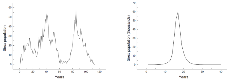
FIGURE 5. Wasp population when dispersal is at random ( P_{LDD}=1 ). For \tau=6 (left plate, a) outbreaks are not observed, but the population cycles and may persist at very low numbers for long periods. For \tau=12 (right plate, b) outbreaks take place soon after wasp introduction. In both cases the initial proportion of susceptible trees ( \rho ) was set to 0.05.
