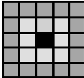
FIGURE 1. Schematic representation of R -neighborhood of a focal tree (black box in the center). The first eight neighboring cells represent the case R=1 (light gray boxes). Adding the outermost 16 cells (dark gray boxes) shows the case R=2 .
