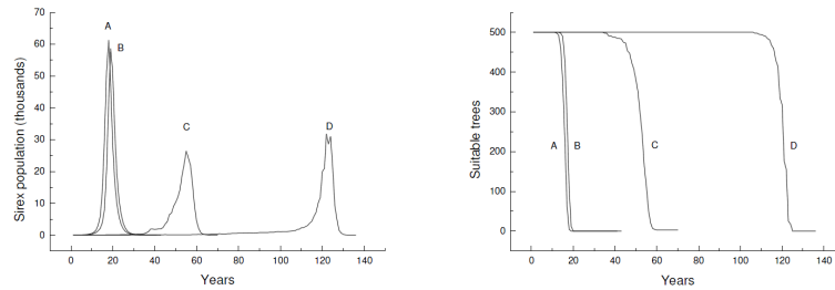
FIGURE 4. (a) Outbreaks obtained for a long distance dispersal probability P_{LDD}=0.1 . Curves A, B, C, and D are as defined in Fig. 3. (b) Dynamics of the population of susceptible trees in the four simulations (A, B, C, and D). In all cases the initial proportion of susceptible trees ( \rho ) was set to 0.05.
