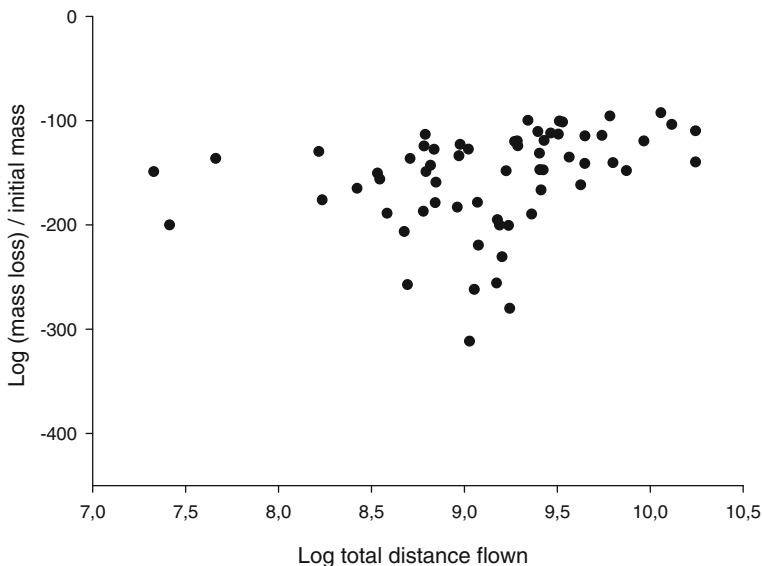
Fig. 2 Female body mass loss during flight trials plotted against total distance flown (m, log-transformed). The total body mass change was estimated as \log(\text{initial mass} - \text{final mass}) / \text{initial mass}
