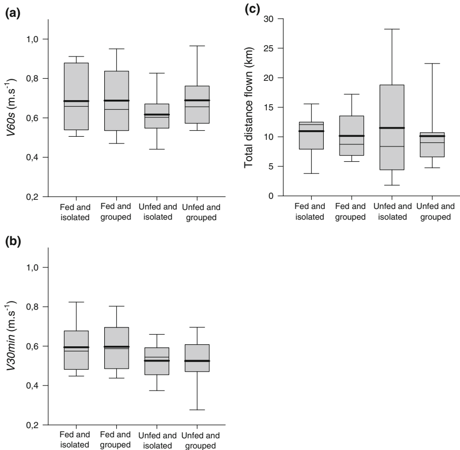
Fig. 1 Flight parameters of I. leucospoides females according to the factorial design; a V60s , b V30min and c total distance flown. Flight parameters studied were neither affected by feeding nor by conspecifics (backward linear model: P<0.005 ). The thin horizontal line of each box plot marks the median of the sample and the thick horizontal line marks the mean of the sample
