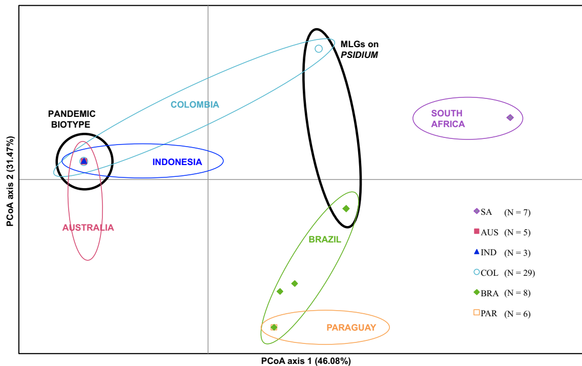
Fig. 2 Principal Coordinates Analysis of 58 isolates of Austropuccinia psidii from different hosts in the Southern Hemisphere. The two axes explain 77.55% of the observed variation based in a covariance matrix with data standardization. Purple diamonds correspond to the South African (SA) samples, red squares to the Australian isolates (AUS), blue
