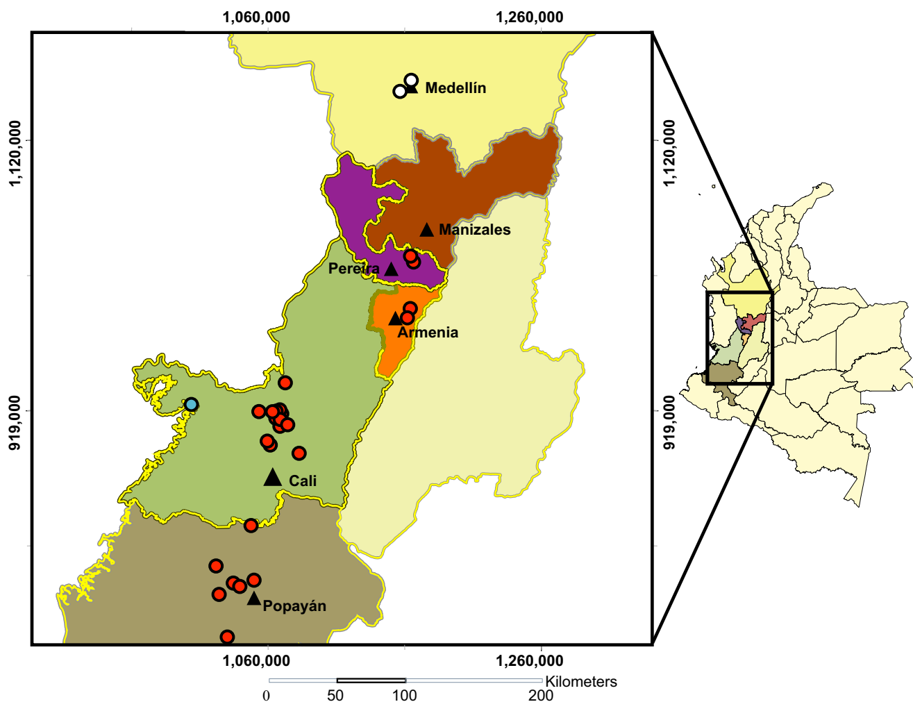
Fig. 1 Geographic distribution of Austropuccinia psidii in Colombia. Red dots represent the surveys. White dots are from first reports of A. psidii in the early 1920s from the Antioquia province. Additionally,
