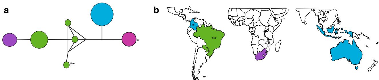
Fig. 3 Graphic representation of the different populations of A. psidii and their location. a Median-joining network of 58 isolates of A. psidii , the size of the circles is proportional to the frequency of different Multilocus genotypes (MLG), the colour represents each of the sampling sites. b
