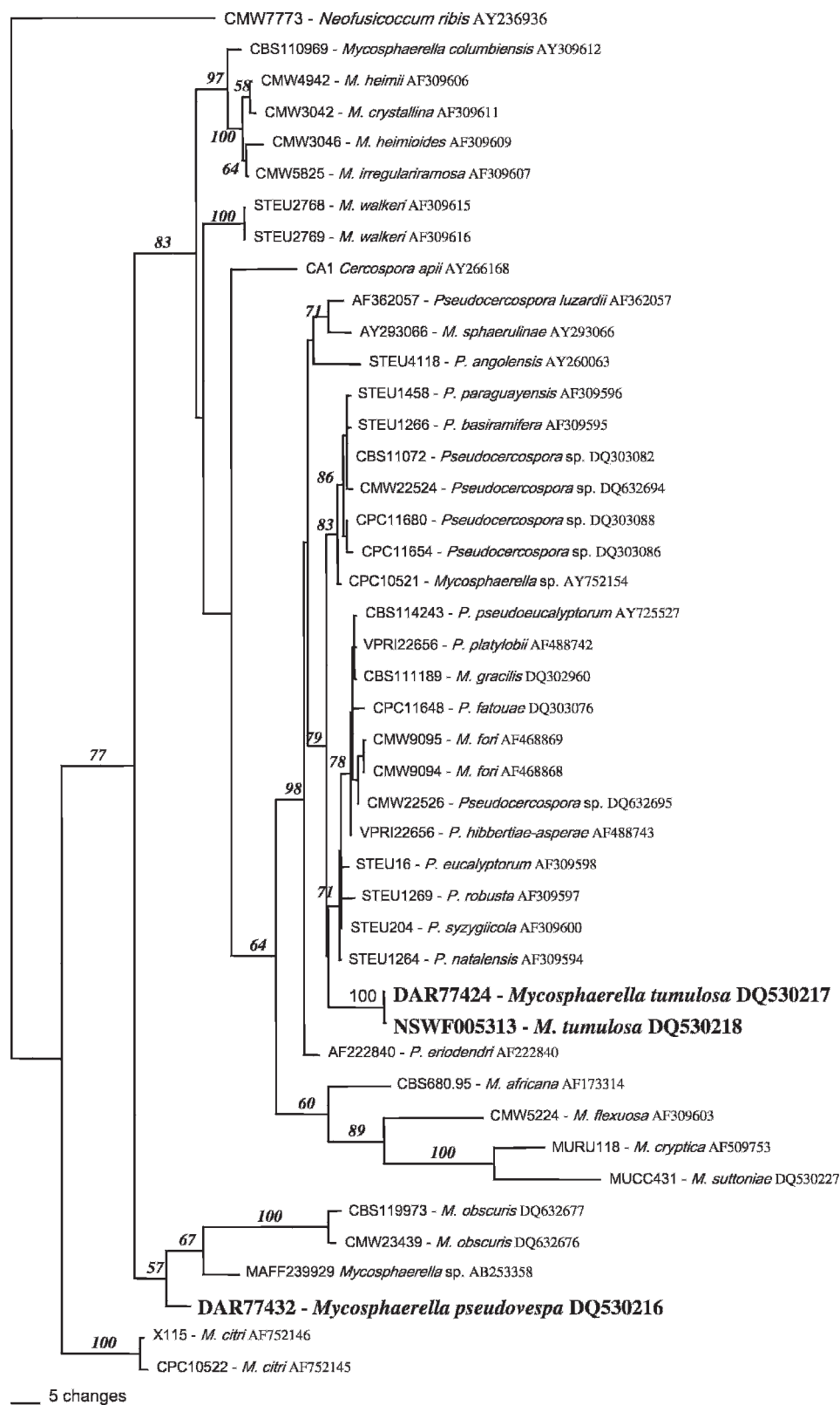
FIG. 2. A phylogram of one of the 30 most parsimonious tree of 348 steps obtained from ITS sequence data, indicating the placement of two new Mycosphaerella spp. in bold. Bootstrap support is given above the branches. The trees were rooted to Neofusicoccum ribis .
