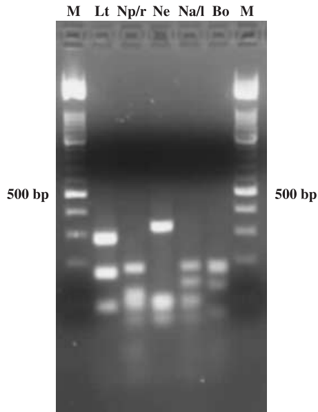
Figure 10 Example of PCR-RFLP fingerprints produced from the ITS1, 5-8S and ITS2 region of Botryosphaeria spp. that occur in South Africa, using the RE CfoI . Lt = Lasiodiplodia theobromae ; Np/r = N. ribis/N. parvum (I or II); Ne = N. eucalyptorum ; Na/l = N. luteum/N. australe (III or IV); Bo = ' Botryosphaeria obtusa ' (VIII). 100 bp markers (M) are run on either side.
