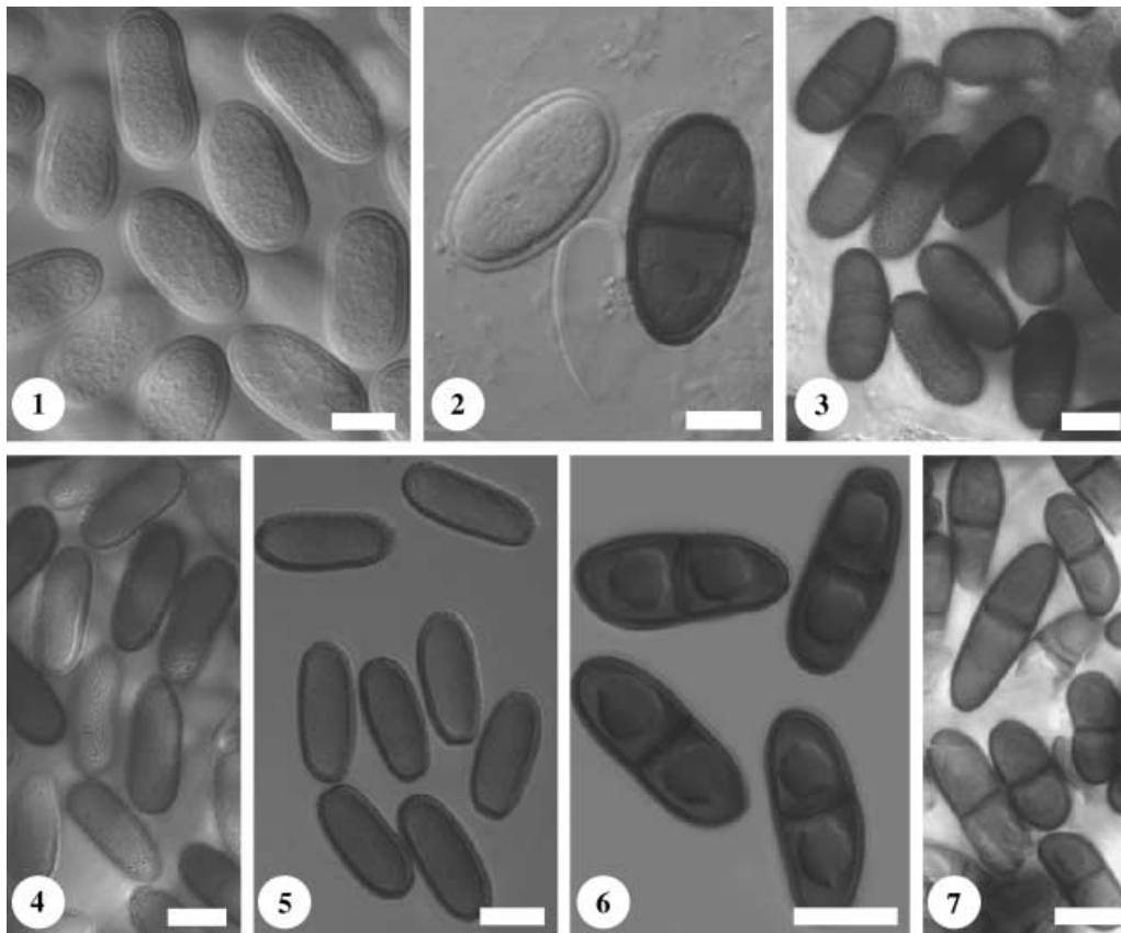
Figures 1–7 DIC compound-microscope micrographs of some anamorphs of Botryosphaeria spp. 1–2: Hyaline, aseptate and pigmented, septate conidia of D. mutila . 3–5: Hyaline and pigmented, aseptate conidia, as well as pigmented, 1–2-septate conidia with rough walls of the Diplodia anamorph of ' Botryosphaeria obtusa '. 6–7: Dark, septate conidia from herbarium material of Diplodia malorum . There were two types of conidia: sample A, shown in Fig. 6 and sample B, shown in Fig. 7 (see text). Bars = 10 µm.
