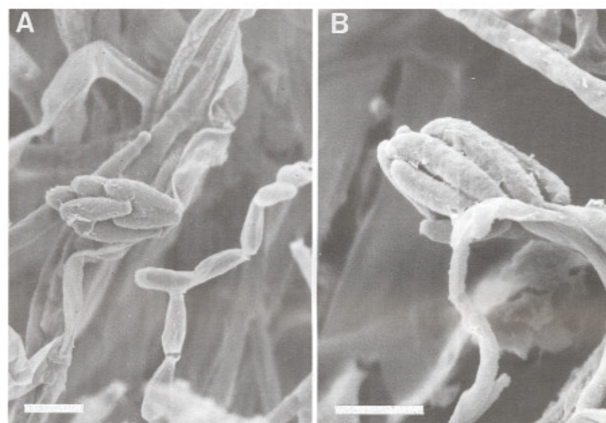
Fig. 1. Scanning electron micrograph of the microconidial ontogeny of (A) Fusarium proliferatum (M-668), producing microconidia in false heads and chains, and (B) F. subglutinans (MRC 6217), producing microconidia in false heads only. Scale bar = 5 \mu m.
