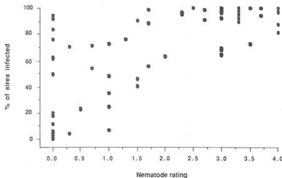
Figure 1: Plot of mean nematode rating from woodchips and percentage of sirex infected with nematodes for observations from the lower, mid, upper, and top strata with more than 10 sirex dissected ( n = 76 ).
