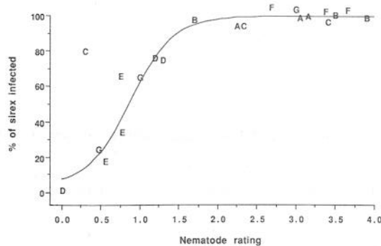
Figure 2: Plot of mean nematode rating from woodchips and percentage of sirex infected with nematodes for tree observations ( n = 21 ). Letters denote the compartments. A logistic curve was fitted to these data (except Tree 9 from Cpt C).
