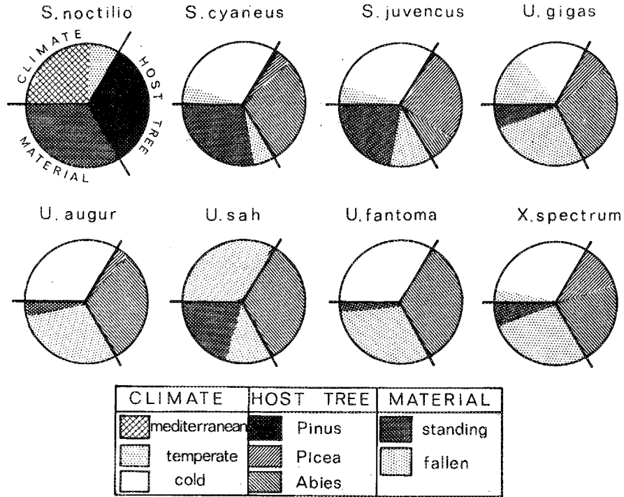
Fig. 6.—Distribution of siricid woodwasps in relation to climate, host tree genera and type of infested timber (based on CSIRO survey).
